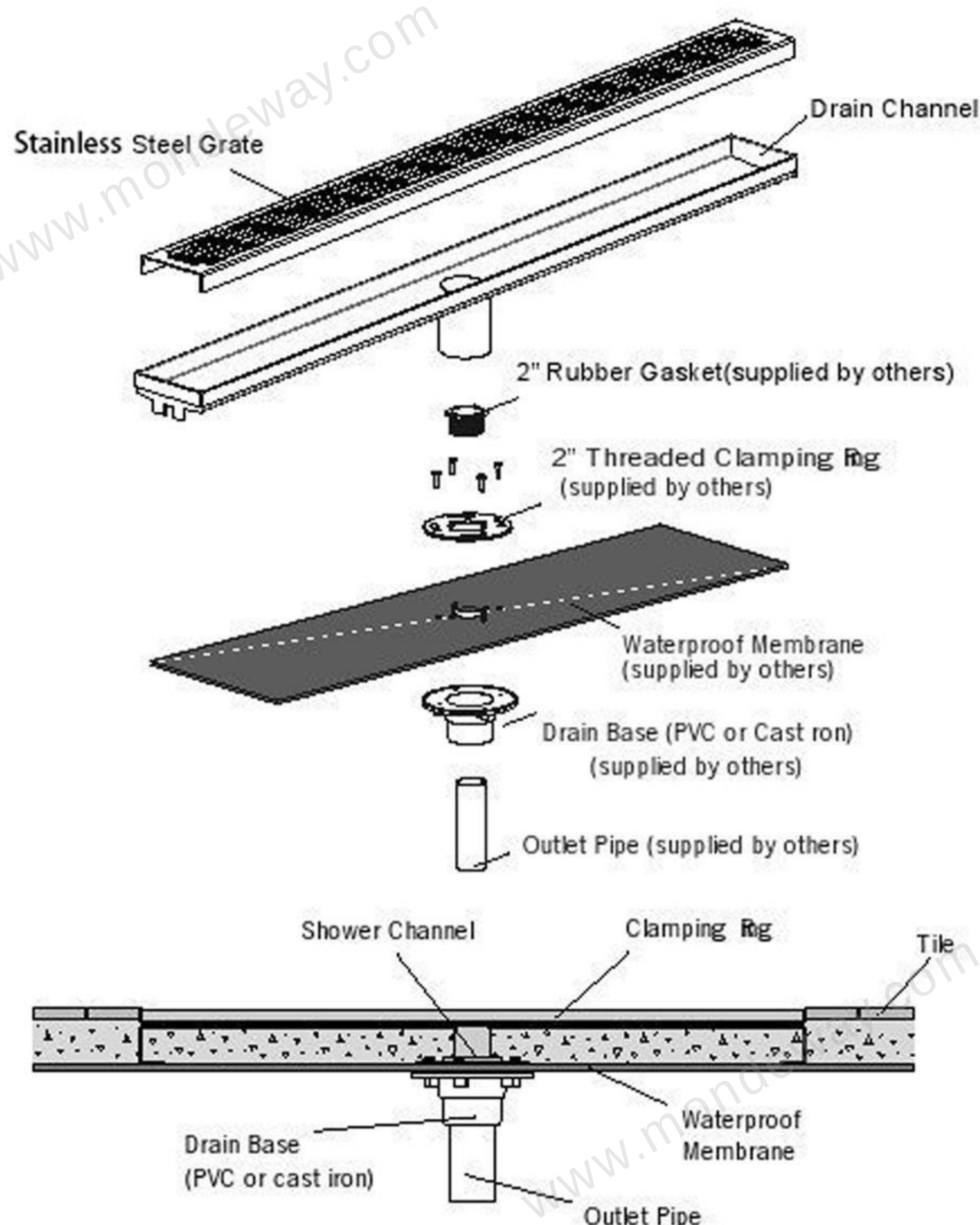
Exploded view of the typical linear drain components.
